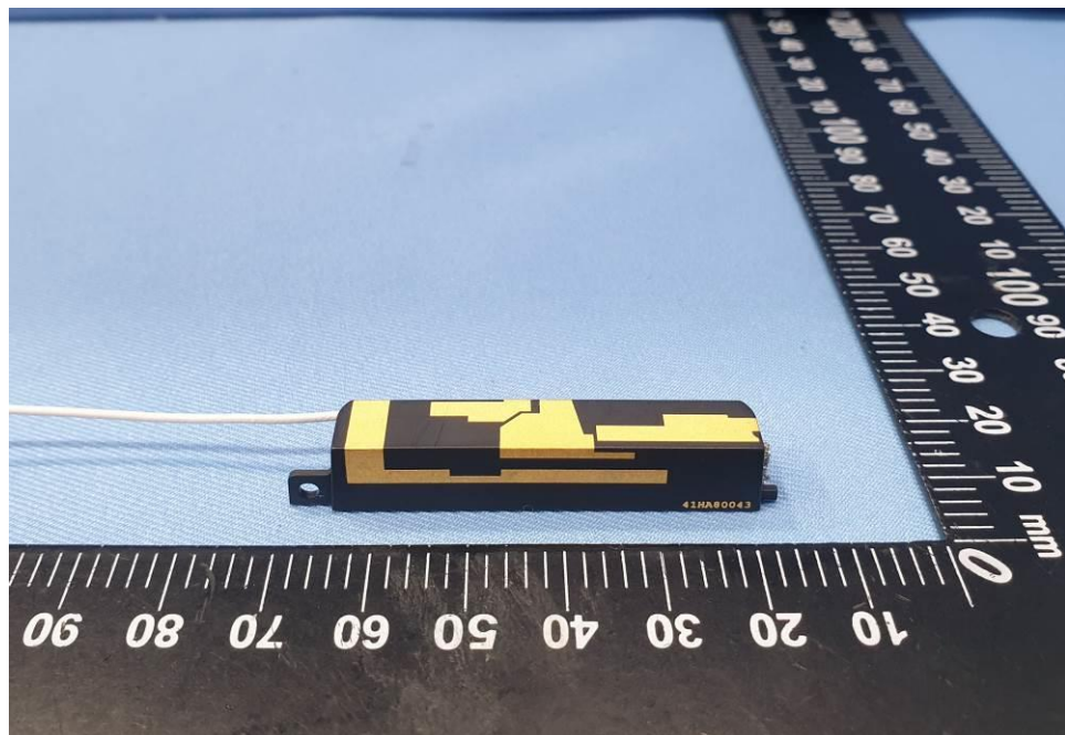
EUT Photo (76)
