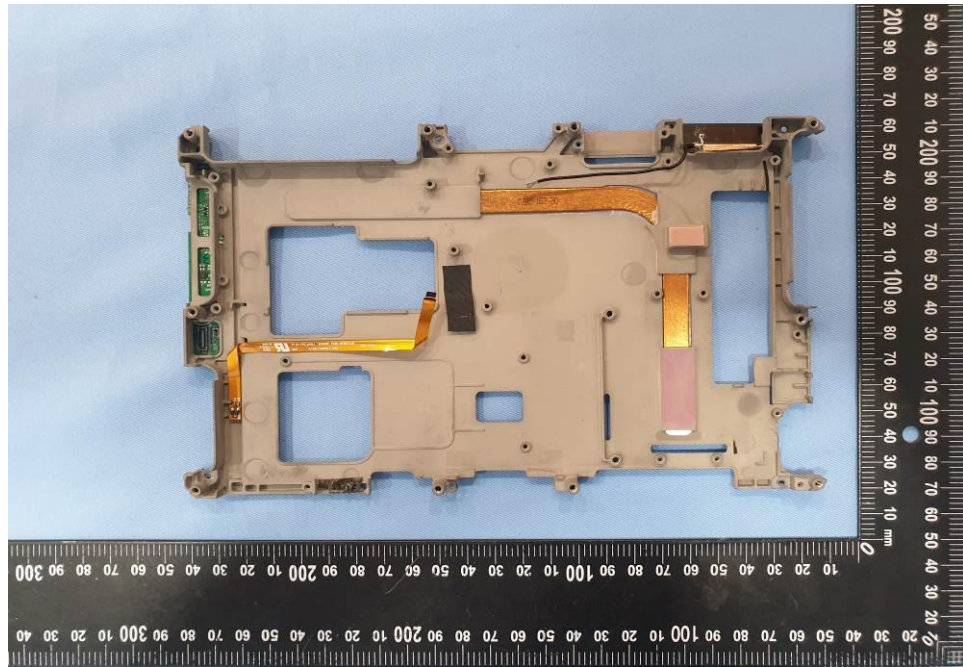
EUT Photo (80)
