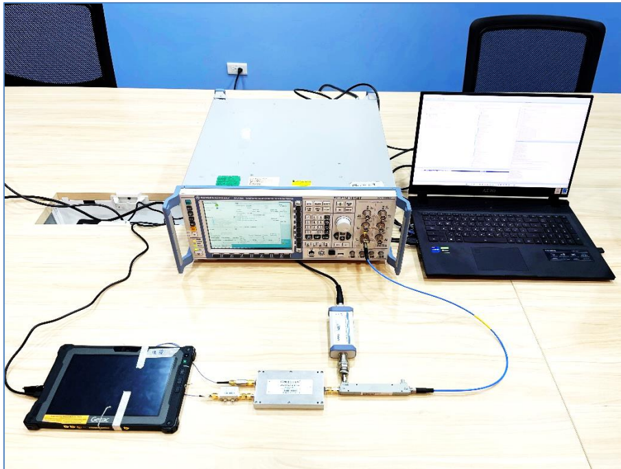
Setup for Conducted Power Testing (Figure 4-5)
