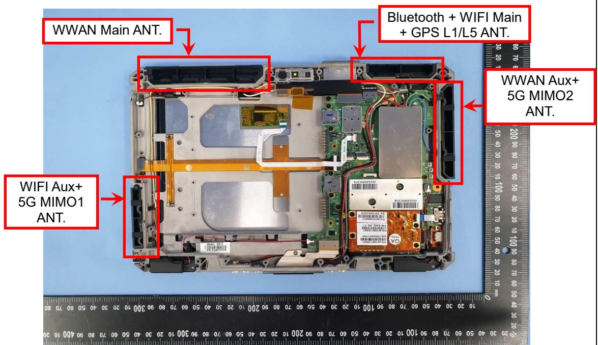
EUT Photo (22)
