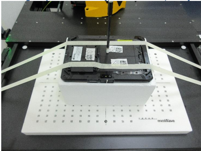
Testing Setup for Power Density, Ant Side at 0 mm, Battery 1
