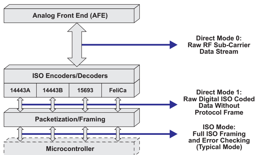
Figure 6-27. User-Configurable Modes
