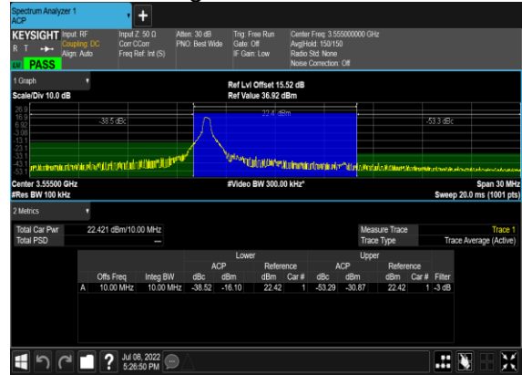
B13_N48(10M)_DFT-s-OFDM_QPSK_Outer_Full_Low_CH
