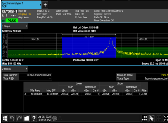
B13_N48(10M)_DFT-s-OFDM_PI_2-BPSK_Edge_1RB_Right_High_CH
