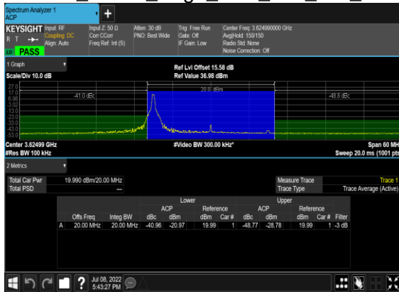
B13_N48(20M)_DFT-s-OFDM_QPSK_Edge_1RB_Left_Mid_CH
