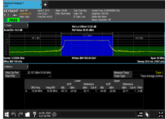
B13_N48(10M)_DFT-s-OFDM_QPSK_Edge_1RB_Right_Low_CH
