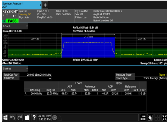
B13_N48(20M)_DFT-s-OFDM_PI_2-BPSK_Edge_1RB_Right_Mid_CH
