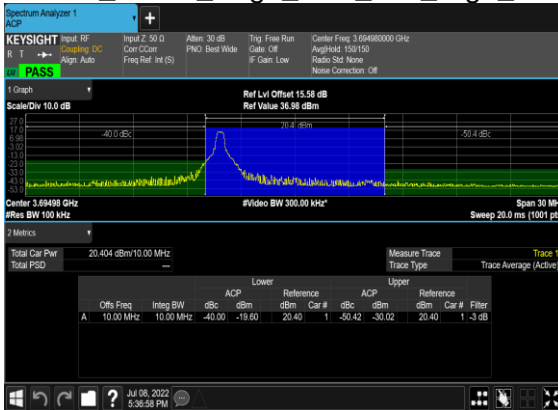
B13_N48(10M)_DFT-s-OFDM_QPSK_Edge_1RB_Left_High_CH
