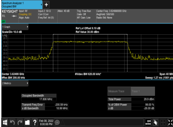
B13_N48(20M)_CP-OFDM_QPSK_Outer_Full_Mid_CH
