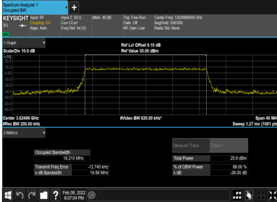
B13_N48(20M)_CP-OFDM_64QAM_Outer_Full_Mid_CH
