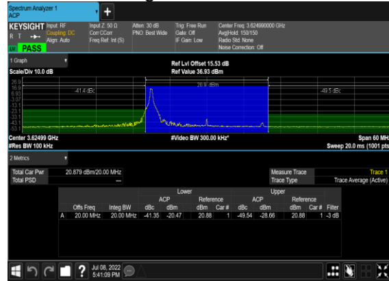
B13_N48(20M)_DFT-s-OFDM_QPSK_Outer_Full_Mid_CH
