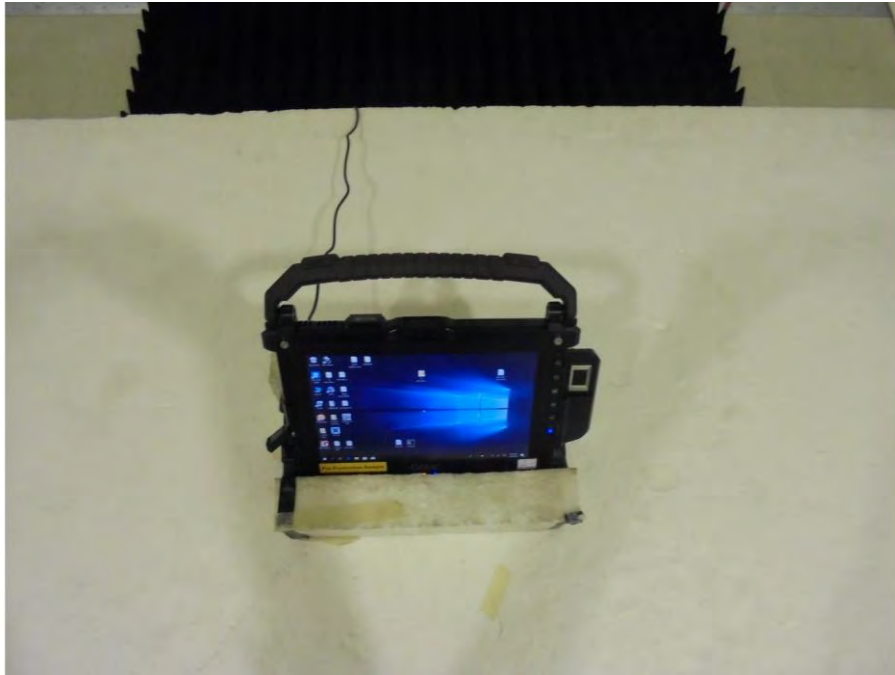
Description: Back View of Radiated Emission Test _ Above 1 GHz
