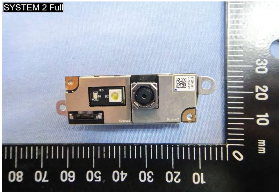
EUT Photo (76)
