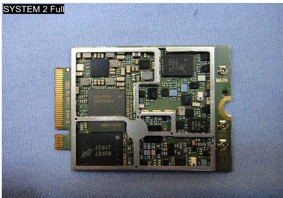
EUT Photo (38)
