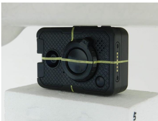
Right Side, Test Separation 25 mm
