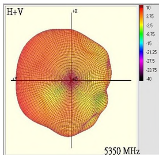
Max Antenna 3D Radiation Pattern 5470-5725 MHz
