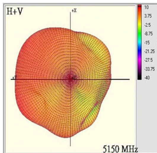
Max Antenna 3D Radiation Pattern 5250-5350 MHz
