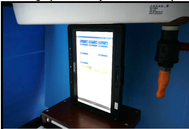
Left Side of EUT with Battery2 Tested at 0 mm
