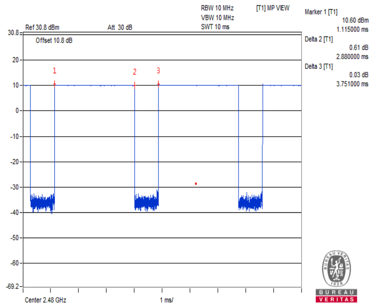
Time-domain plot for Bluetooth transmission signal
