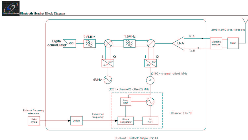
Figure 2: Bluetooth Single Chip IC- Receiver Circuit
