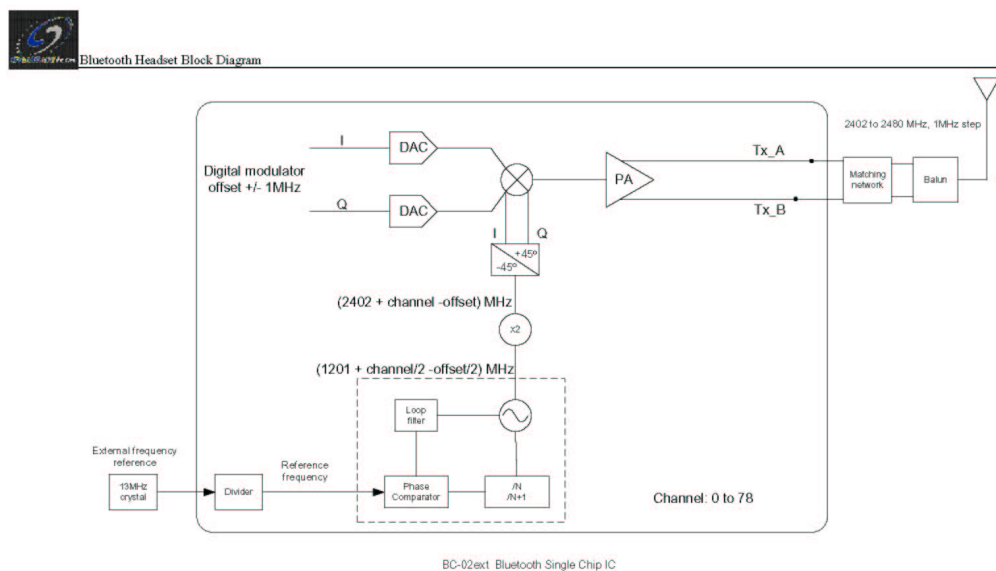
Figure 3 Bluetooth Single Chip IC- Transmitter Circuit
