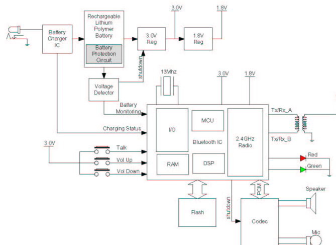
Figure 1: Bluetooth Headset Block Diagram
