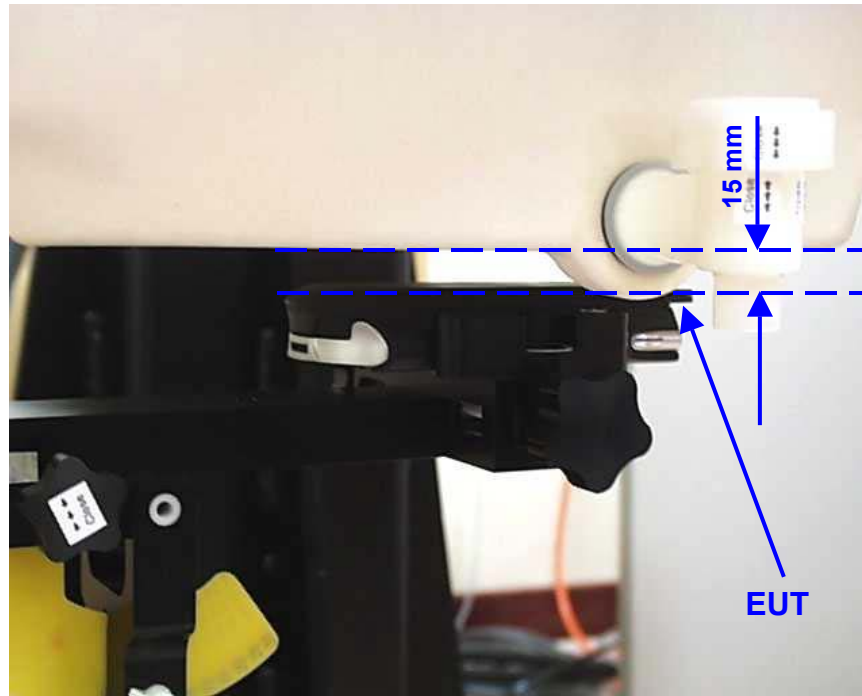
SAR Test Setup At Flat Phantom – Closer View (EUT Rear To Phantom, 15mm spacing)
