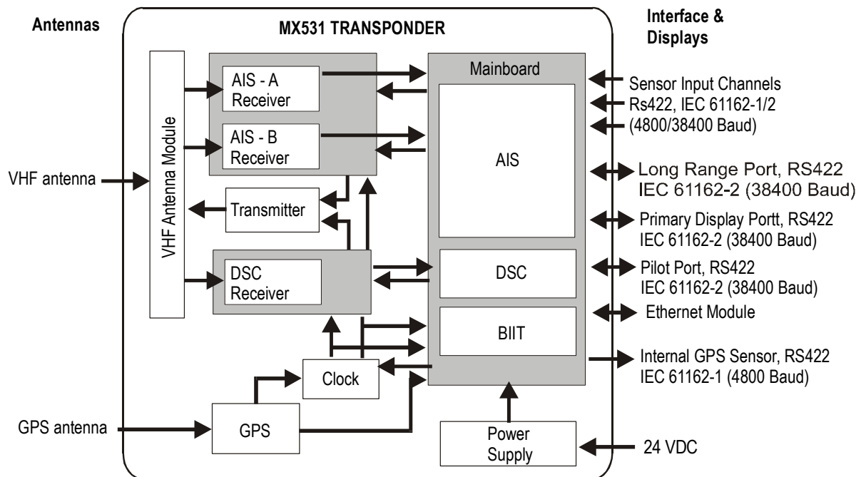
Fig. 4-3 Block diagram of the Transponder Unit
