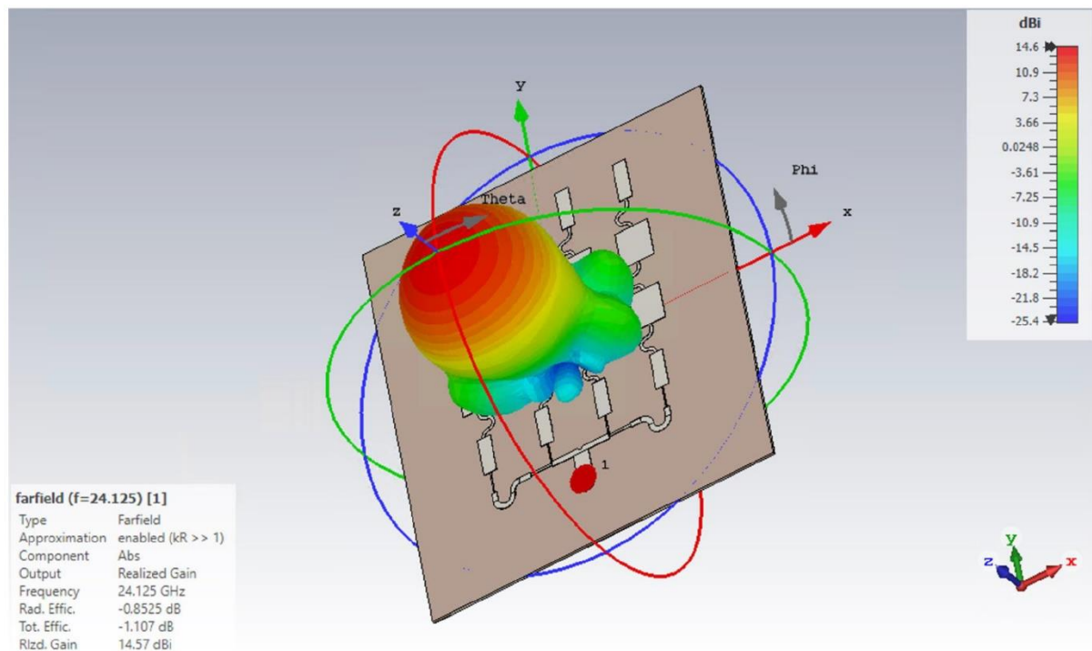
Figure 1 Antenna Radiation Pattern
