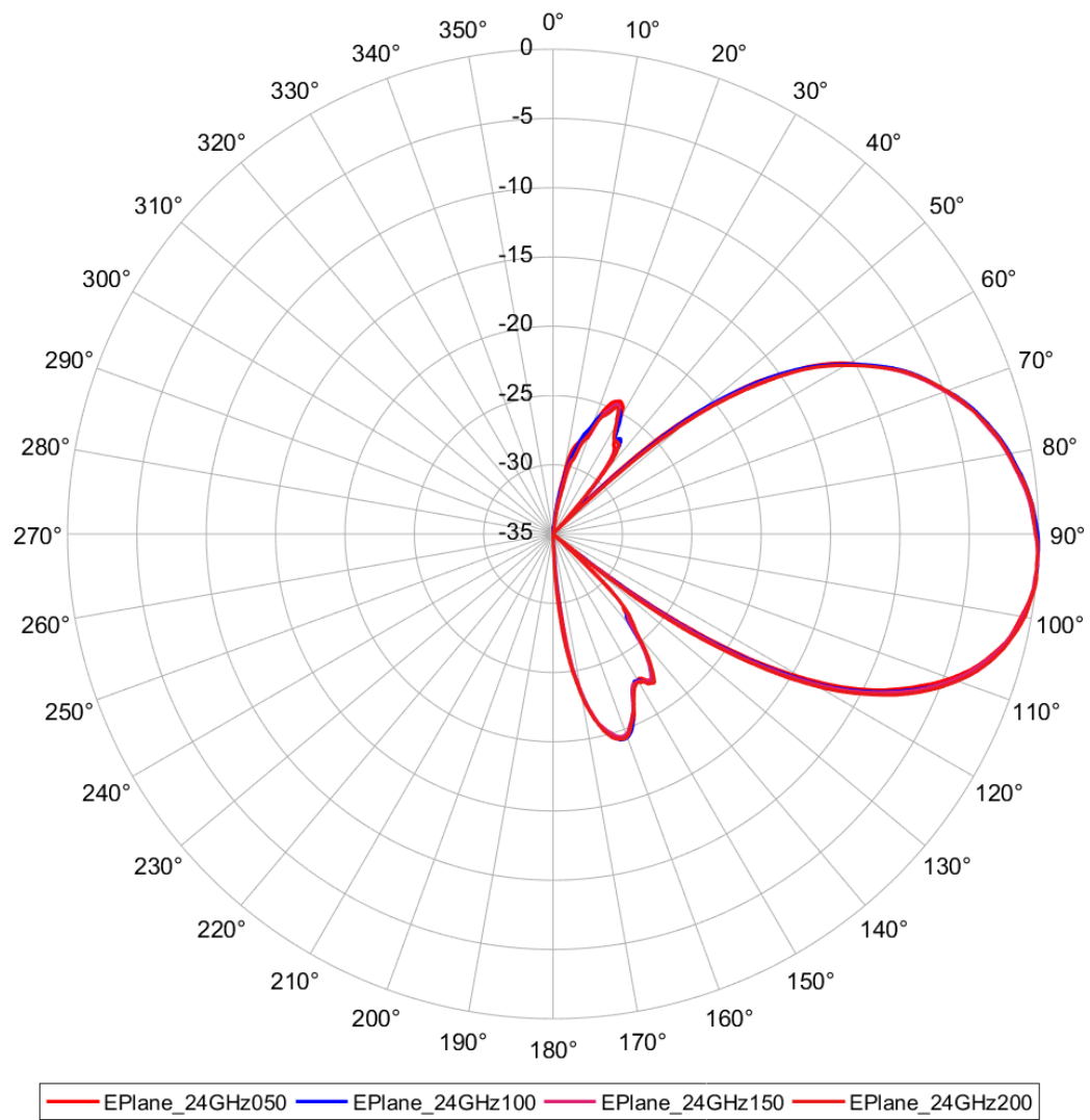
Figure 2 E-plane Radiation Pattern
