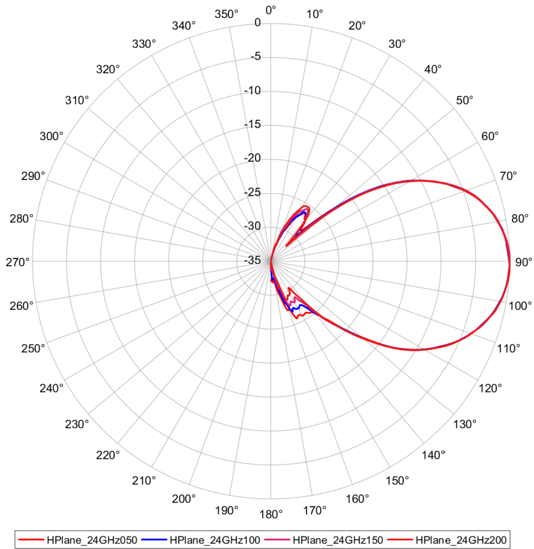
Figure 3 H-plane Radiation Pattern
