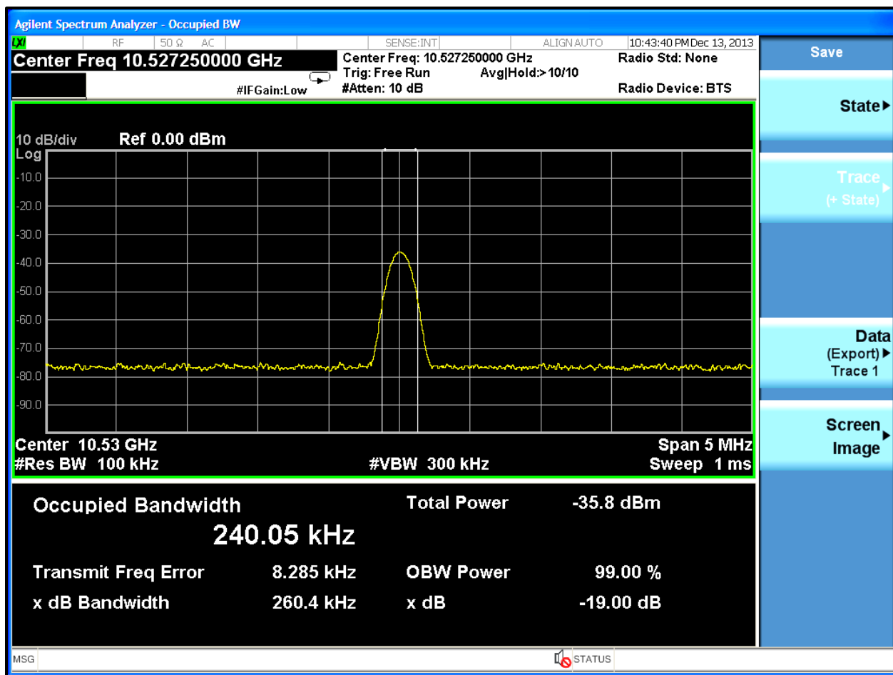
Plot 5-1: 99% Bandwidth
