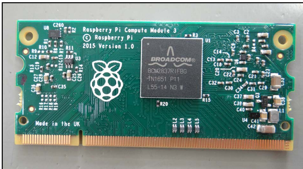
Raspberry Pi Compute Module 3 Top Side
