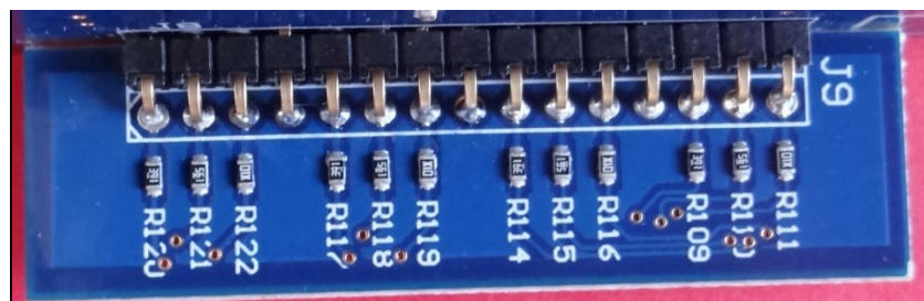
Bottom View of LED PCB fitted to FS MEVO Range PSU &amp; Charger PCB
