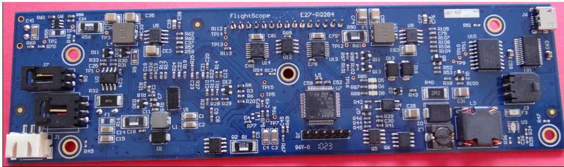
Top View of FS MEVO Range PSU &amp; Charger PCB
