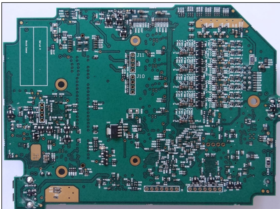
Bottom View of MEVO Range System PCB
