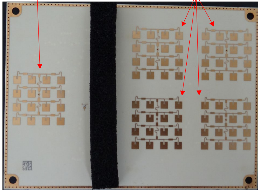
Top View of FS MEVO Range RF PCB
