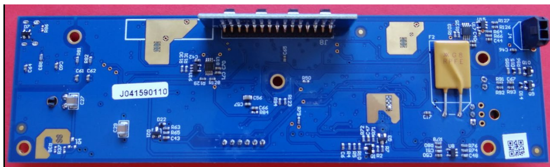
Bottom View of FS MEVO Range PSU &amp; Charger PCB
