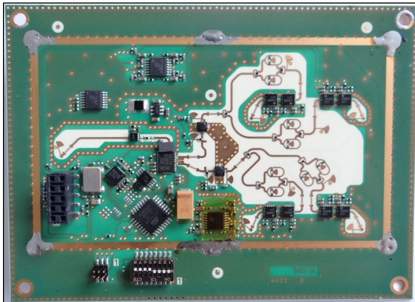
Bottom View of FS MEVO Range RF PCB (Without Shield)
