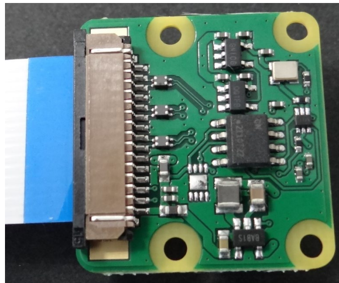
Bottom View of Raspberry PI Camera Module V2
