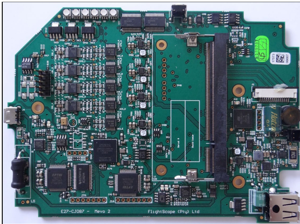
Top View of MEVO Range System PCB
