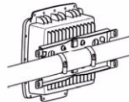
Figure 6 AP3660 - Pole Mount Option 3
