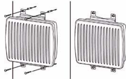
Figure 7 AP3660 - Wall Mount
