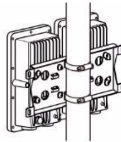
Figure 6 AP3660 Power Supply - Pole Mount Option 2
