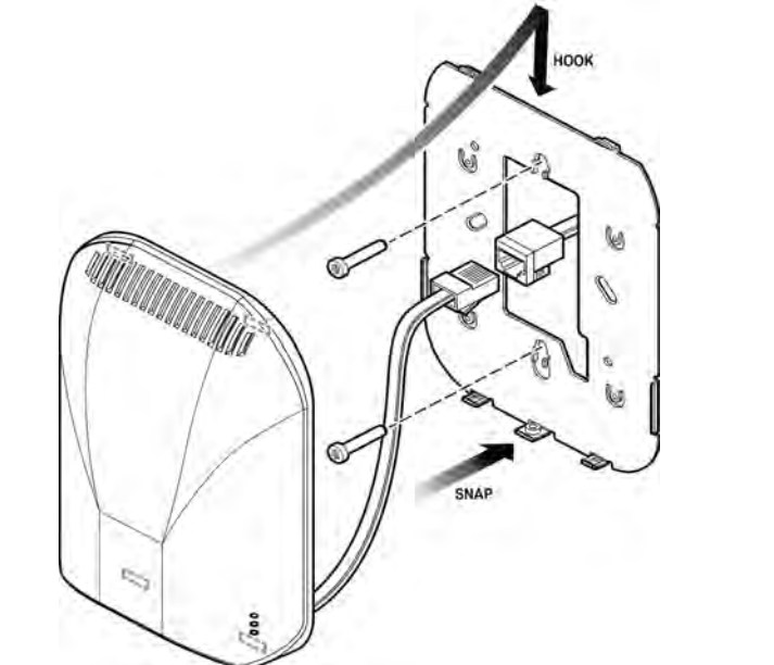
Figure 4 Mounting the AP
