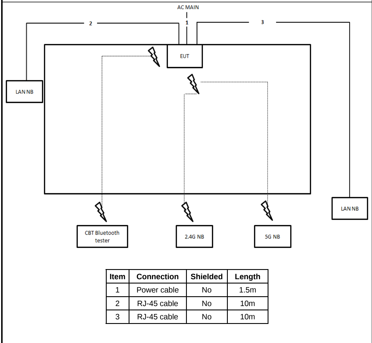
Test Setup Diagram - Radiated Test < 1GHz
