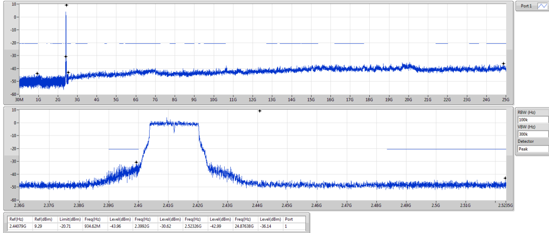
802.11g_Nss1,(6Mbps)_1TX 2412MHz
