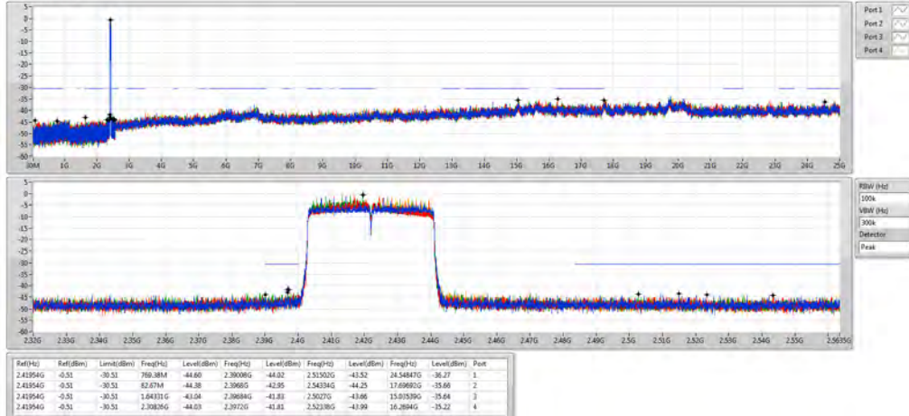
802.11ax HEW40_Nss1,(MCS0)_4TX 2422MHz
