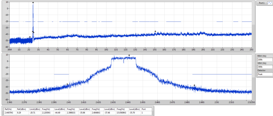
802.11g_Nss1,(6Mbps)_1TX 2437MHz
