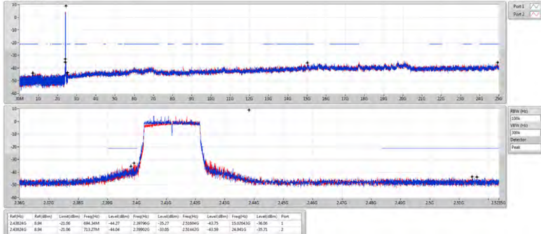
802.11ax HEW20_Nss2,(MCS0)_2TX
