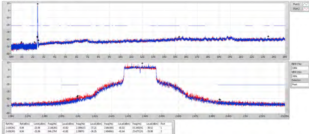
802.11ax HEW20_Nss2,(MCS0)_2TX
