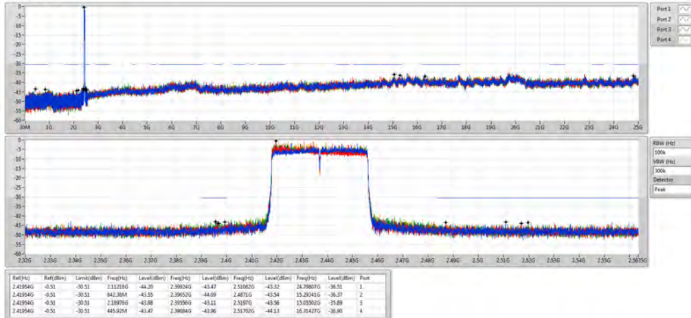
802.11ax HEW40_Nss1,(MCS0)_4TX 2437MHz
