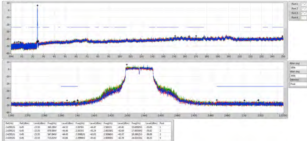
802.11g_Nss1,(6Mbps)_4TX 2437MHz
