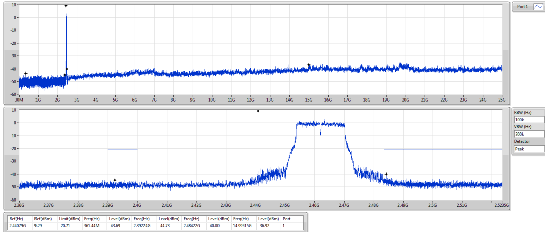
802.11g_Nss1,(6Mbps)_1TX 2462MHz
