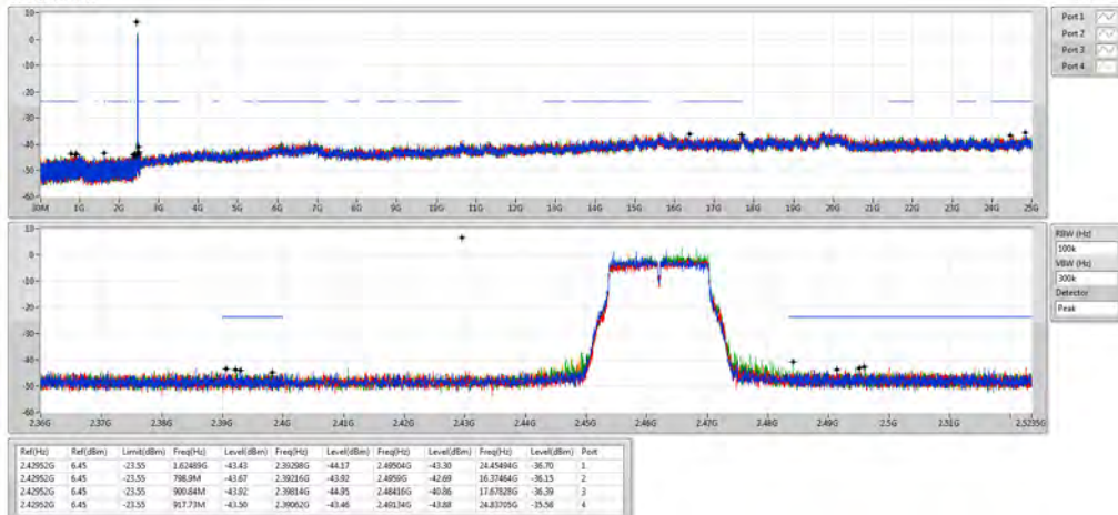
802.11g_Nss1,(6Mbps)_4TX 2462MHz
