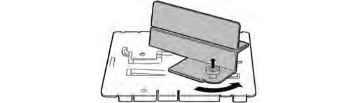
Figure 5 Attaching the adapter to the main bracket
