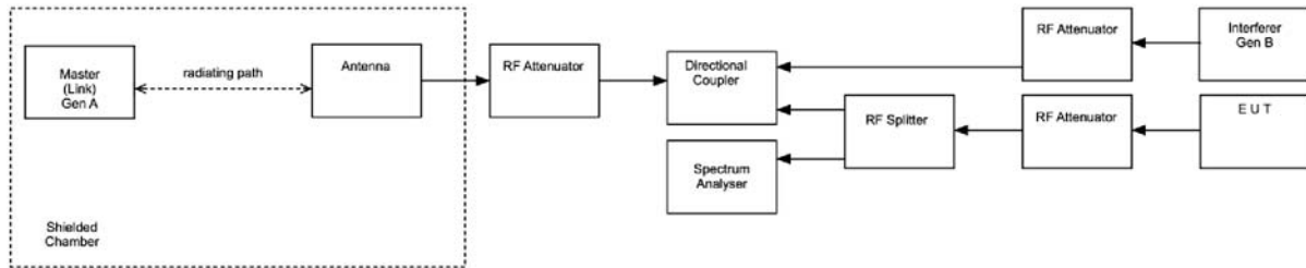
Figure ii Test Setup
