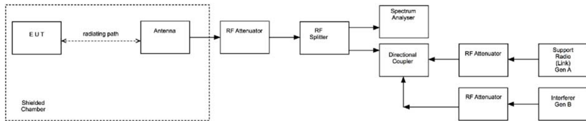
Figure i Test Setup
