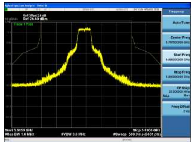
5785MHz with 2*2 CDD PK
