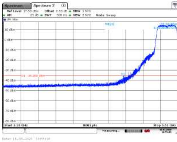
5520MHz with 2*2 Beamforming PK
