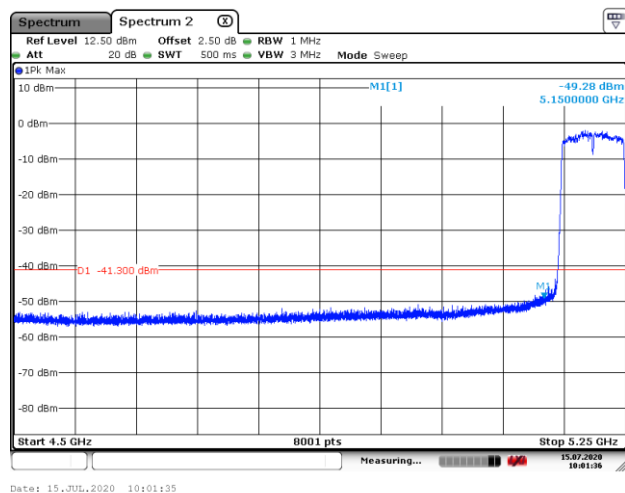
5210MHz with 4*4 Beamforming PK
