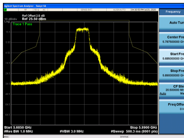
5785MHz with 2*2 Beamforming PK
