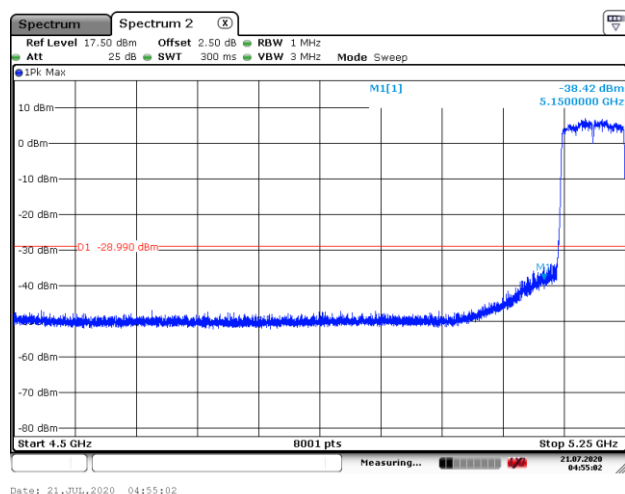
5210MHz with 2*2 CDD PK
