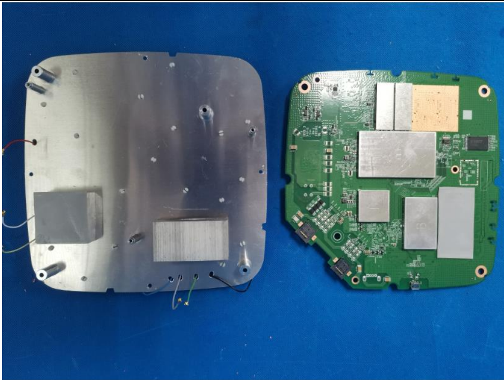
(2) EUT Photo (AP460S6C)
