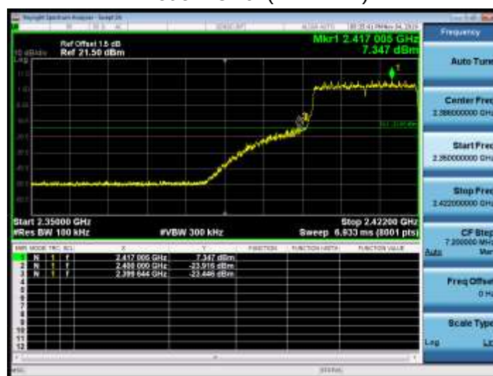
Mode 4 CH01(2412MHz)
