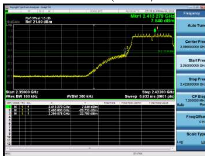
Mode 3 CH01(2412MHz)
