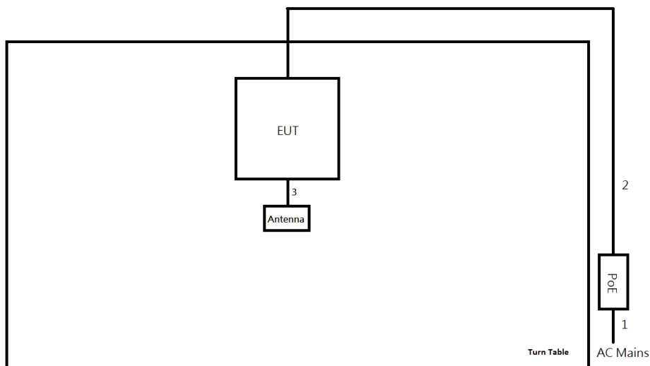
Test Setup Diagram - Radiated Test (Sample 2_Panel 1 Antenna)
