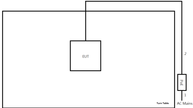
Test Setup Diagram - Radiated Test (Sample 1)
