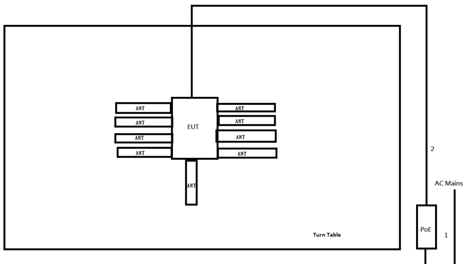
Test Setup Diagram - Radiated Test (Sample 2_Omni)
