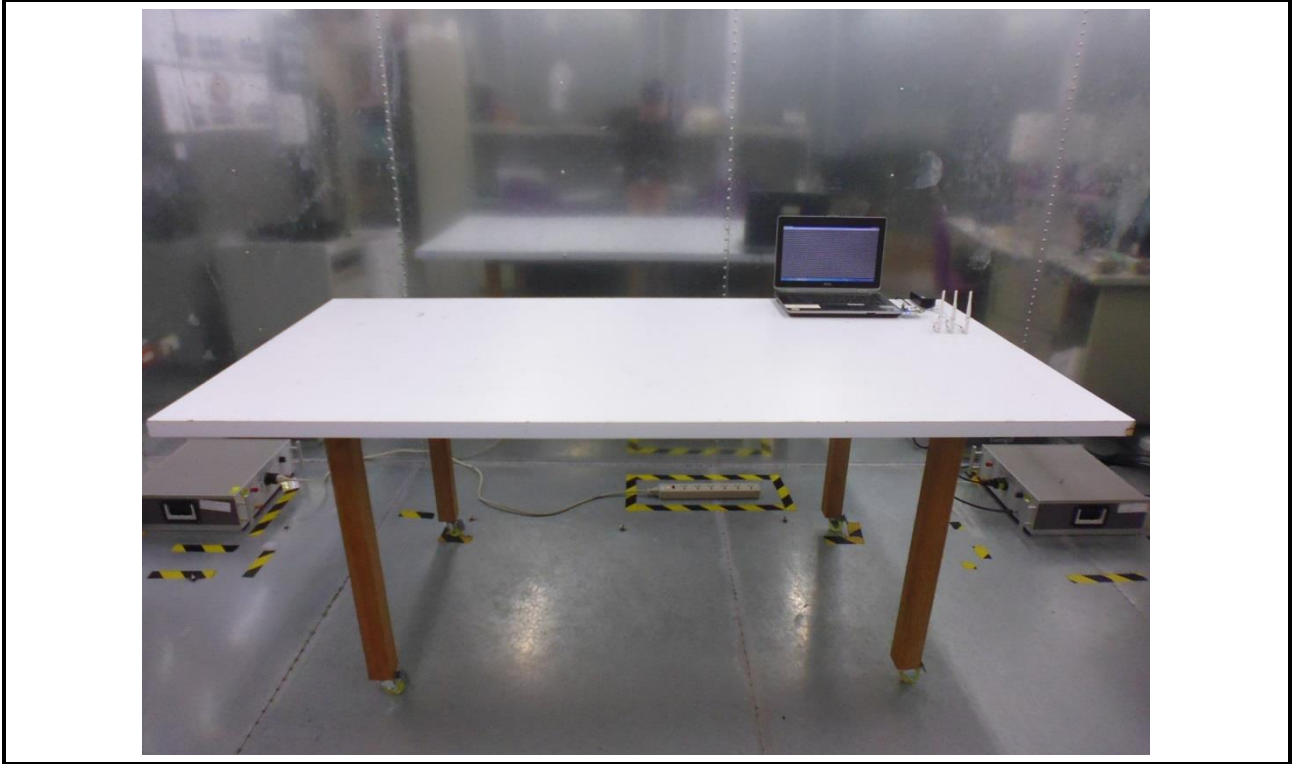
Conducted Emission Test _ Configuration 1
