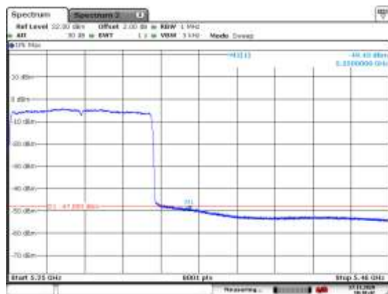
5290MHz with SISO
