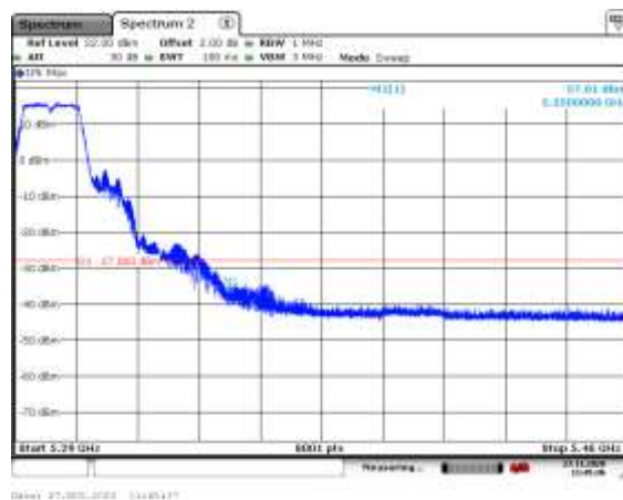
5300MHz with SISO
