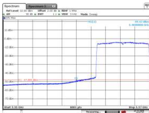
5530MHz with SISO
