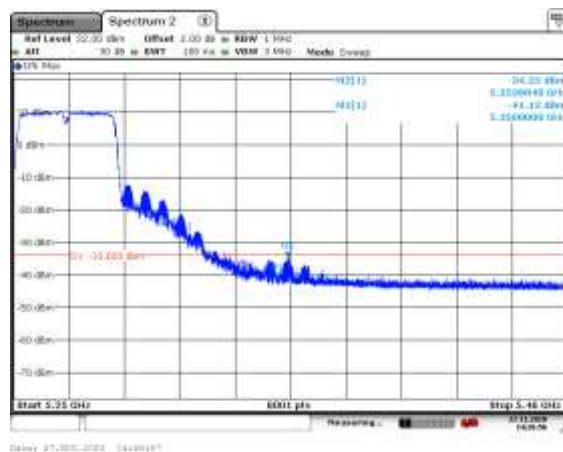
5270MHz with Beamforming
