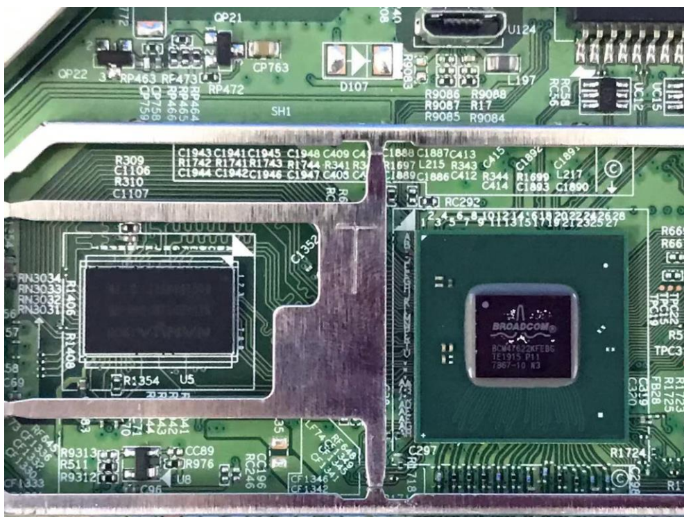
(6) EUT Photo(AP305C)
