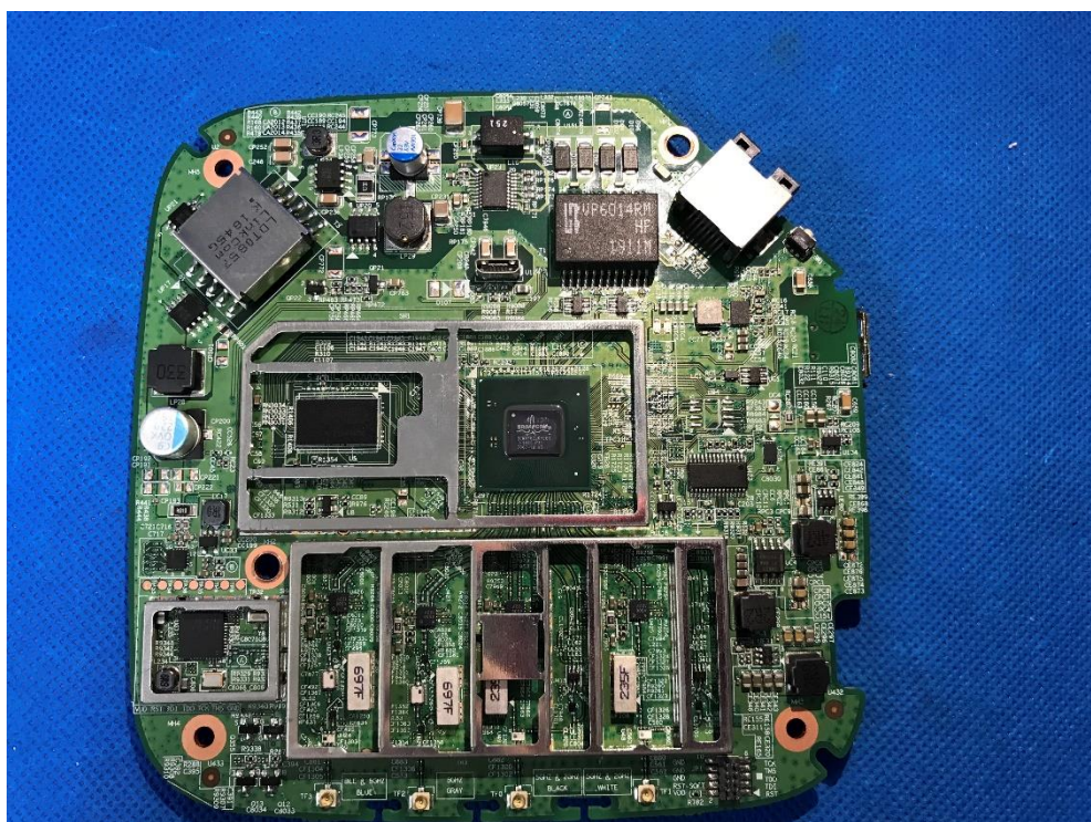
(4) EUT Photo(AP305C)
