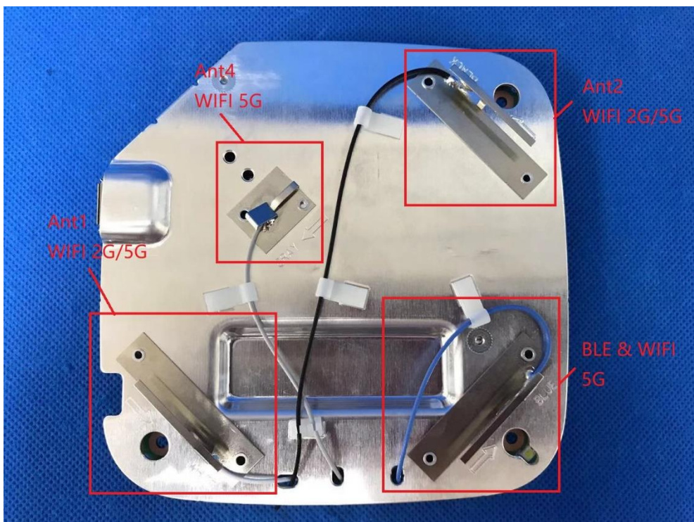
(2) EUT Photo(AP305C)
