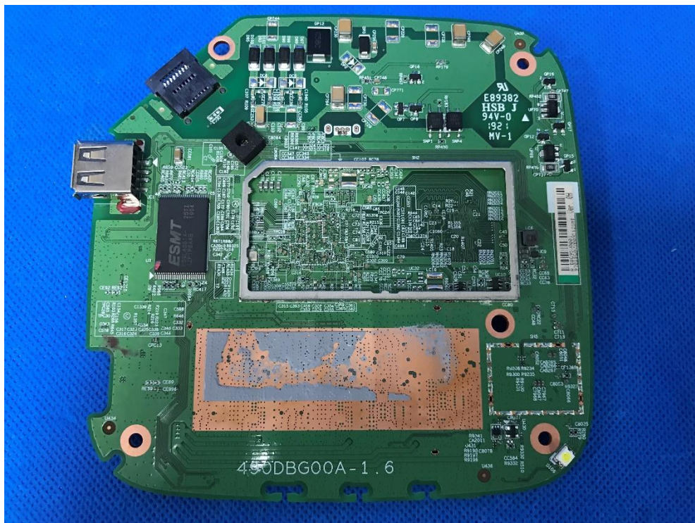
(12) EUT Photo(AP305CX)
