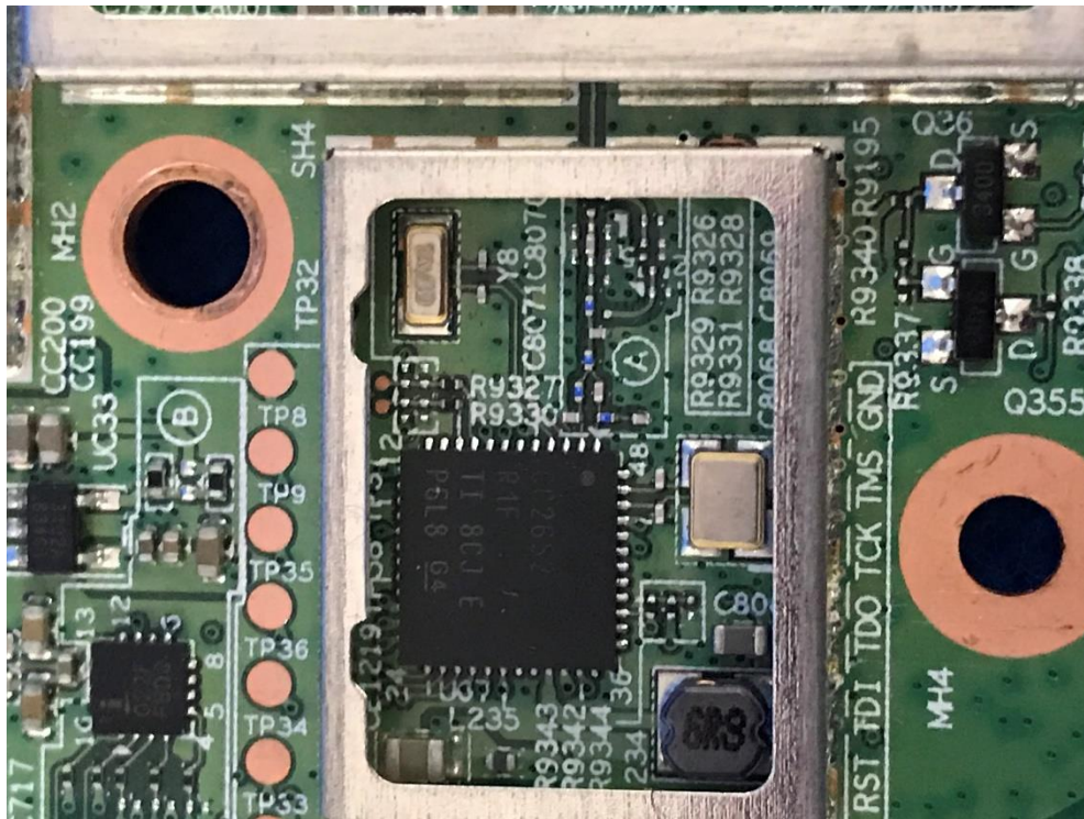
(8) EUT Photo(AP305CX)
