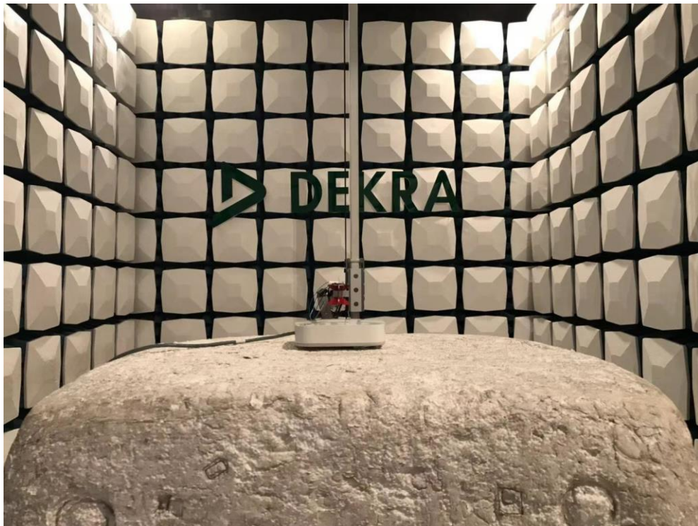
Description: Radiated Emission Test Setup for 1~18GHz(AP305C)
