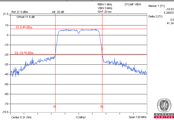
8802.11ac (VHT40)_Chain 0 / CH62
