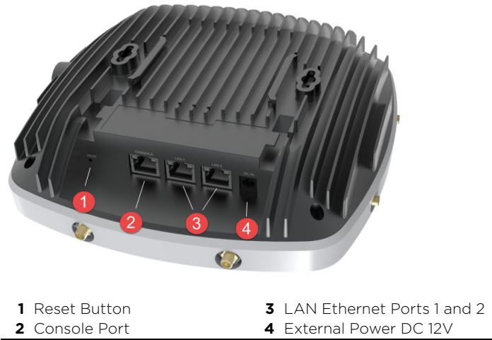
Figure 4 3935e Access Point bottom view
