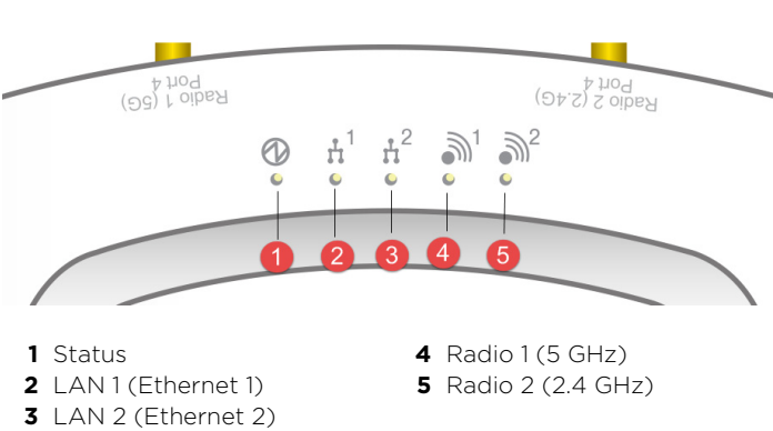
Figure 3 LEDs on AP Front Face
