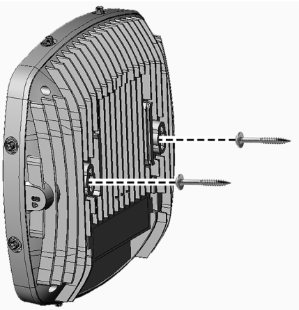
Figure 7 Mounting the AP3935 to a Flat Wall.
