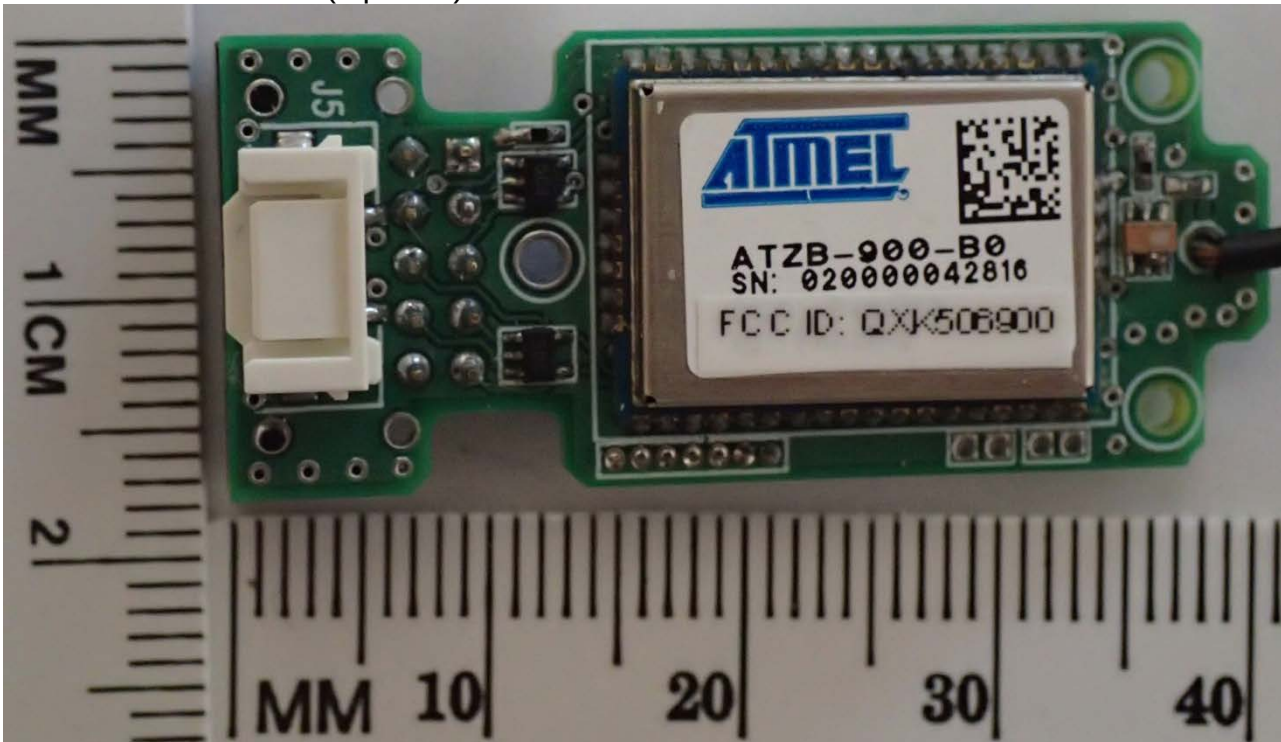
EUT dimensional view (top view)
