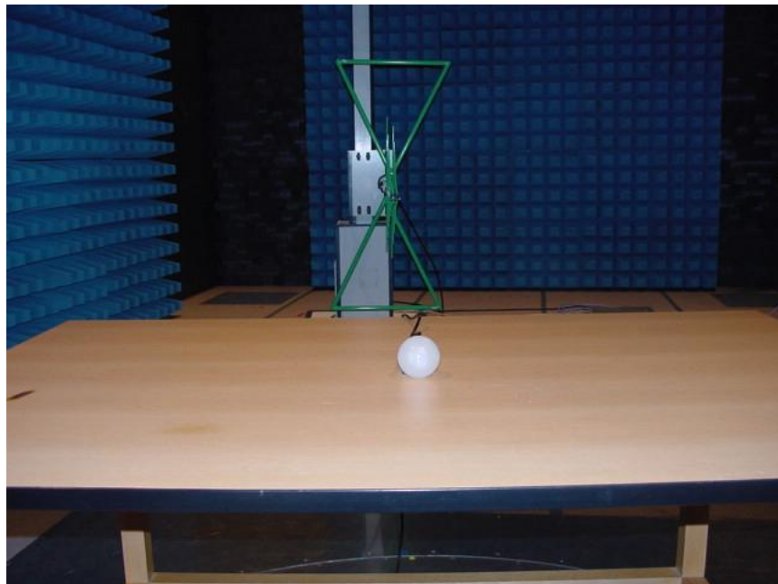
Radiated emission test view for EUB series
