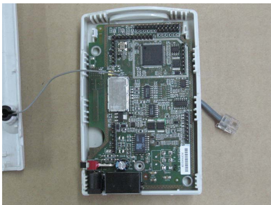
Figure 2 PCB in Cover
