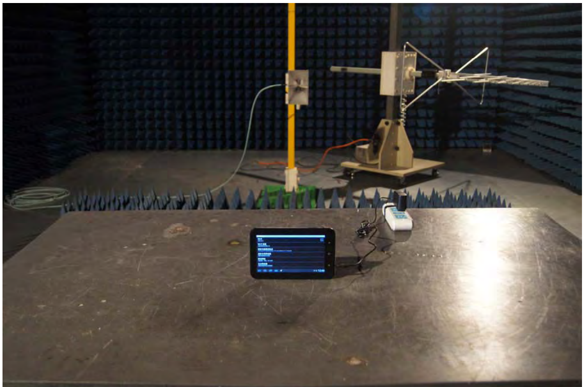
Radiated emissions test > 1GHz (Part 15C)
