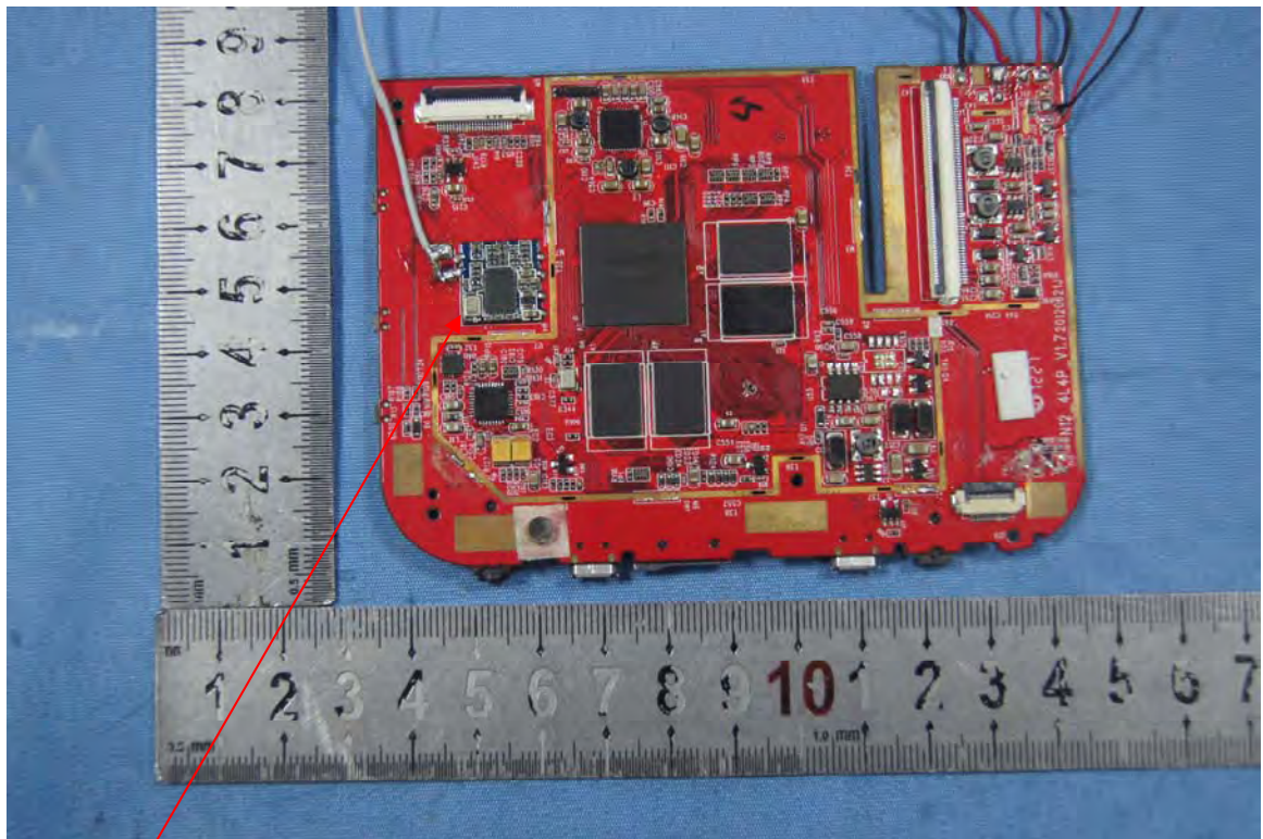
Wireless Module
