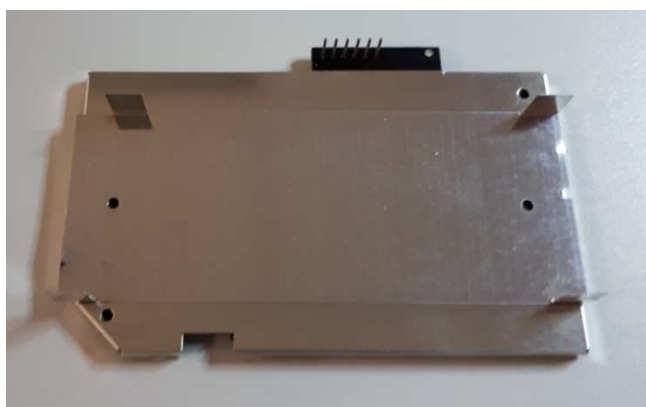
Charging coil element with connector, ferrite plate and metal shield, view from top and bottom side.
