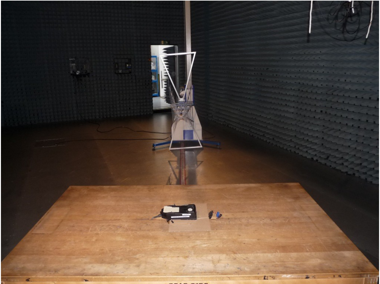
Photo 3: Test setup for spurious radiated emissions measurements (Enclosure, semi-equipped anechoic chamber, 30 MHz -1GHz intentional radiator §15)
