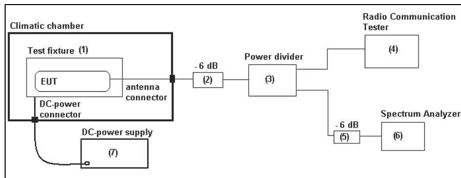
Schematic: Test set-up conducted within climatic chamber
