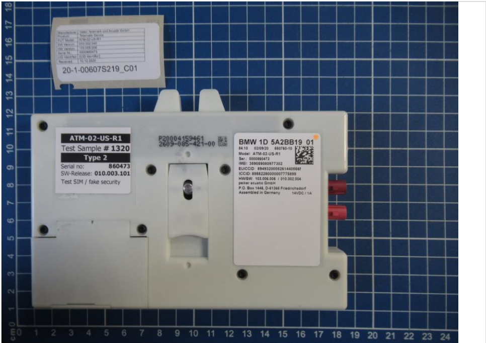
Photograph 5: EUT 2_Top side view
