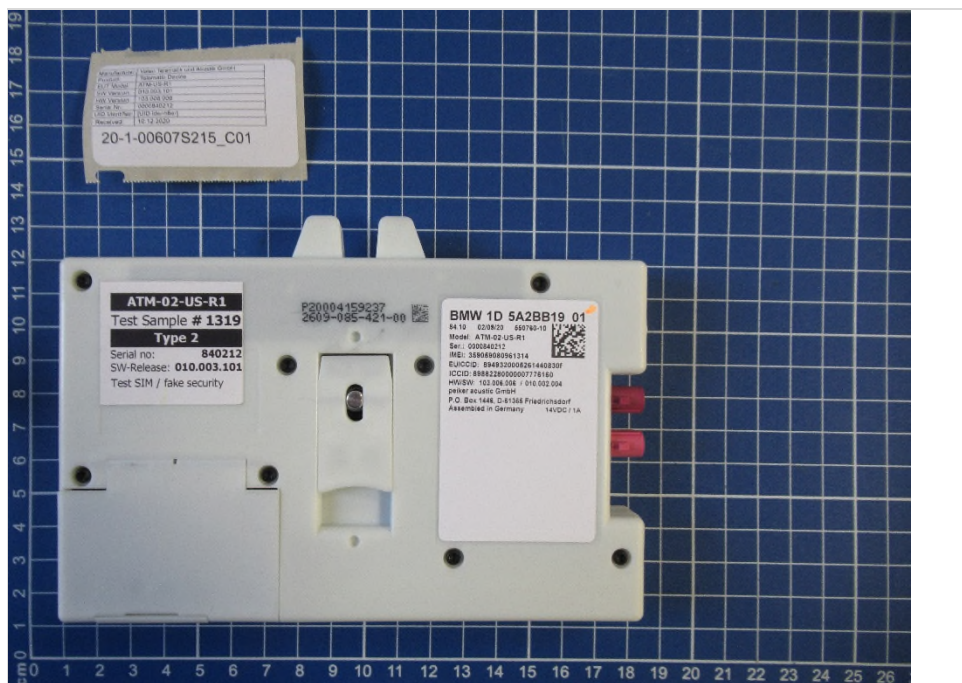
Photograph 2: EUT Top view
